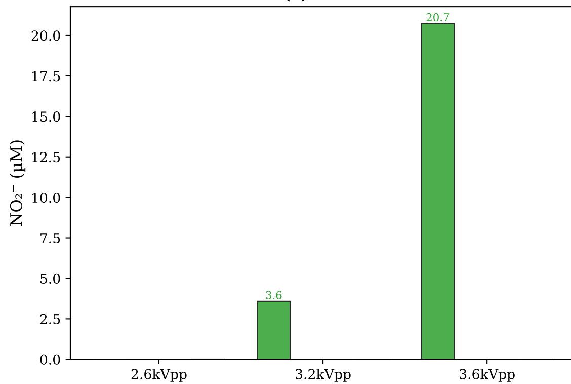
(c) \text{NO}_2^-
